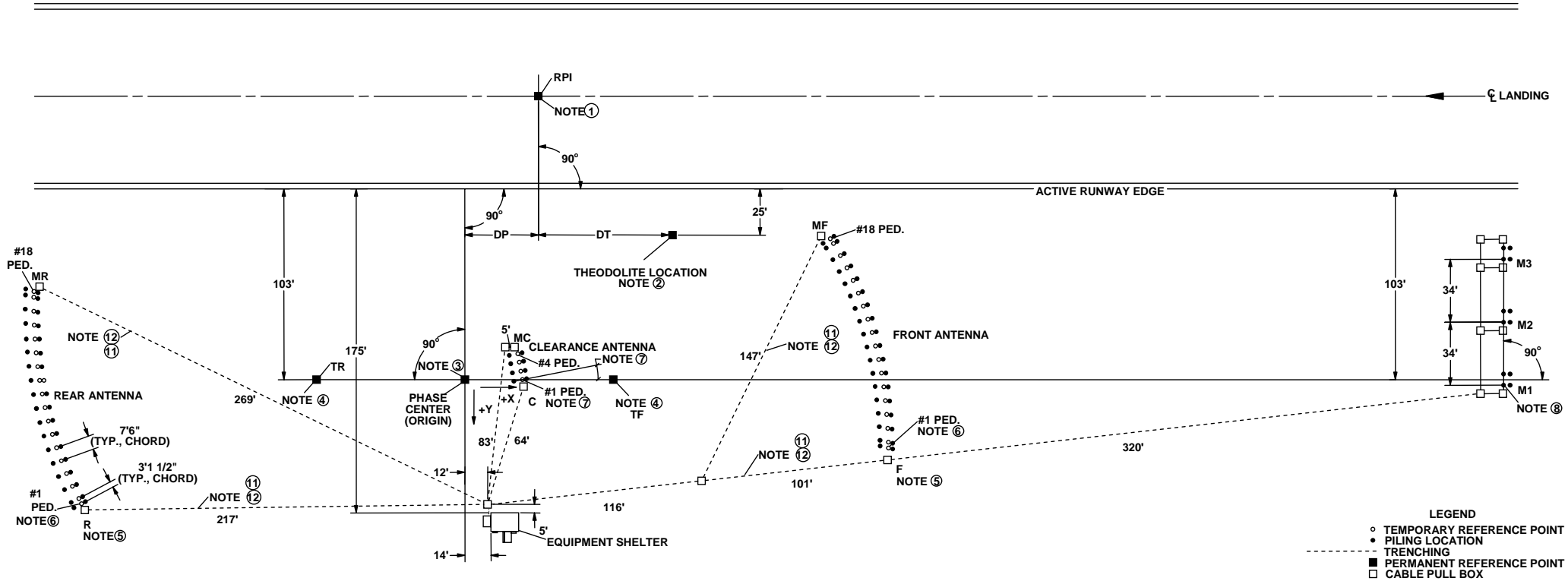
Figure 9-1. Construction Drawing Sheet 1 of 5
