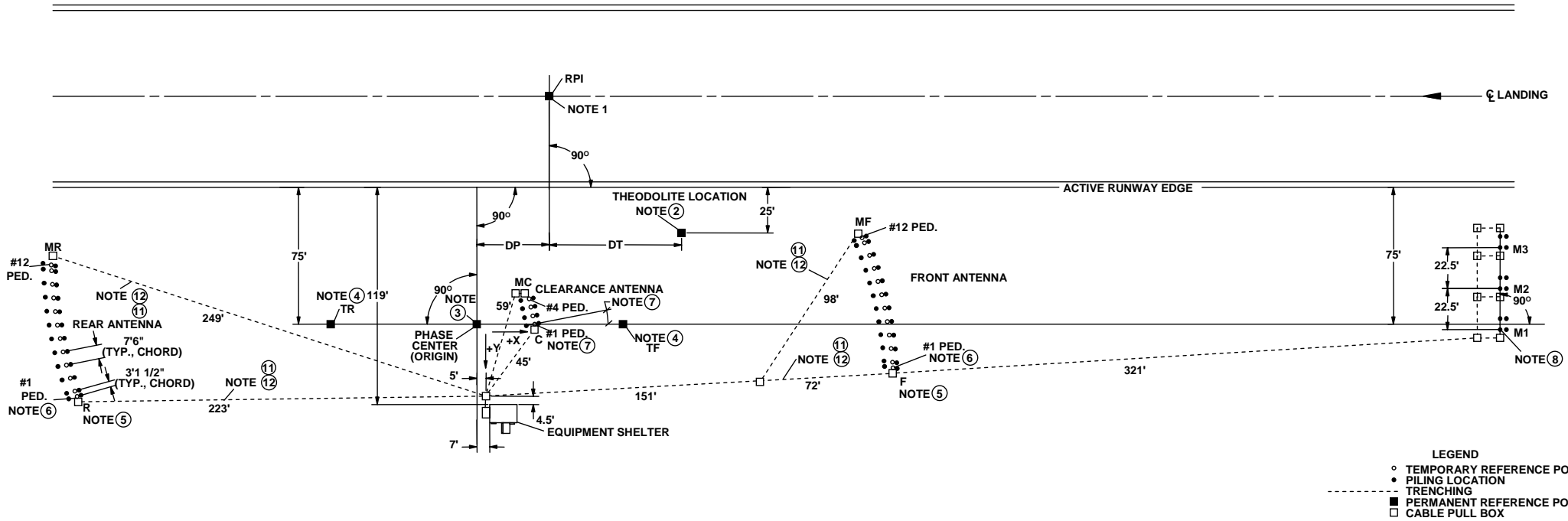
FIGURE 9-1. CONSTRUCTION DRAWING Sheet 1 of 5
